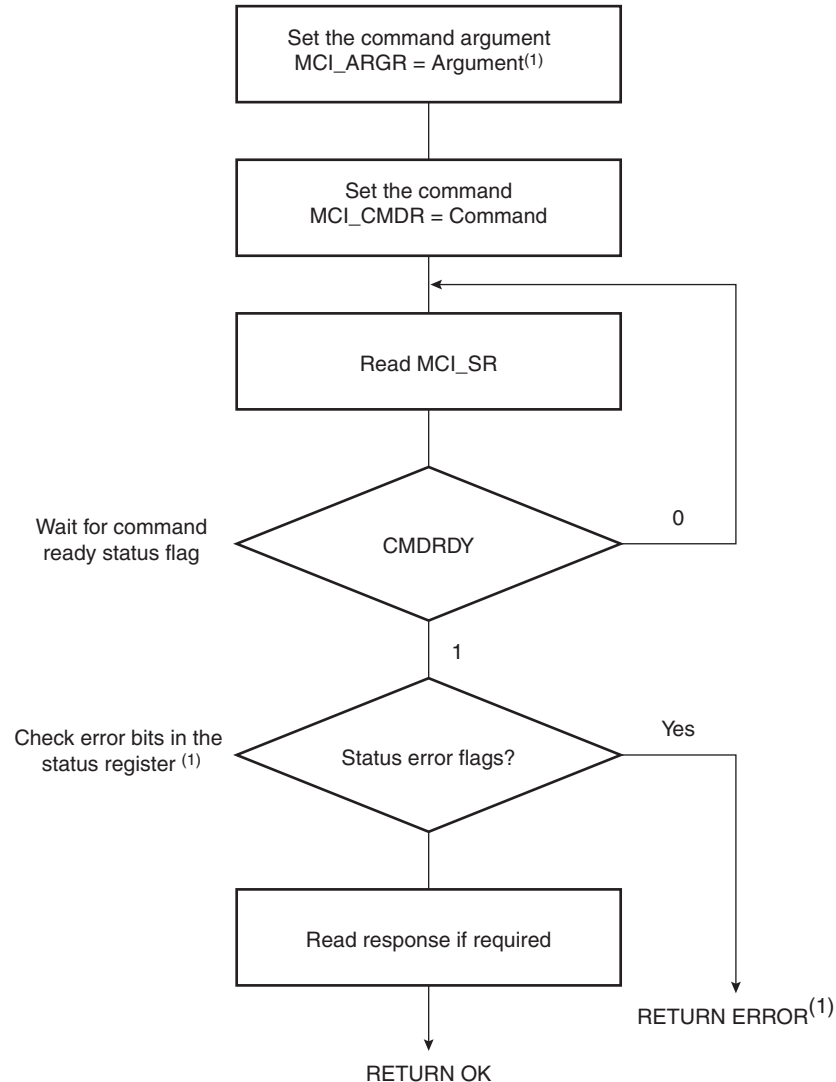
Figure 39-9. Command/Response Functional Flow Diagram
