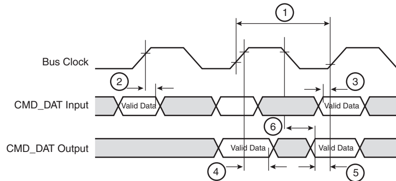
Figure 46-12. MCI Timing Diagram
