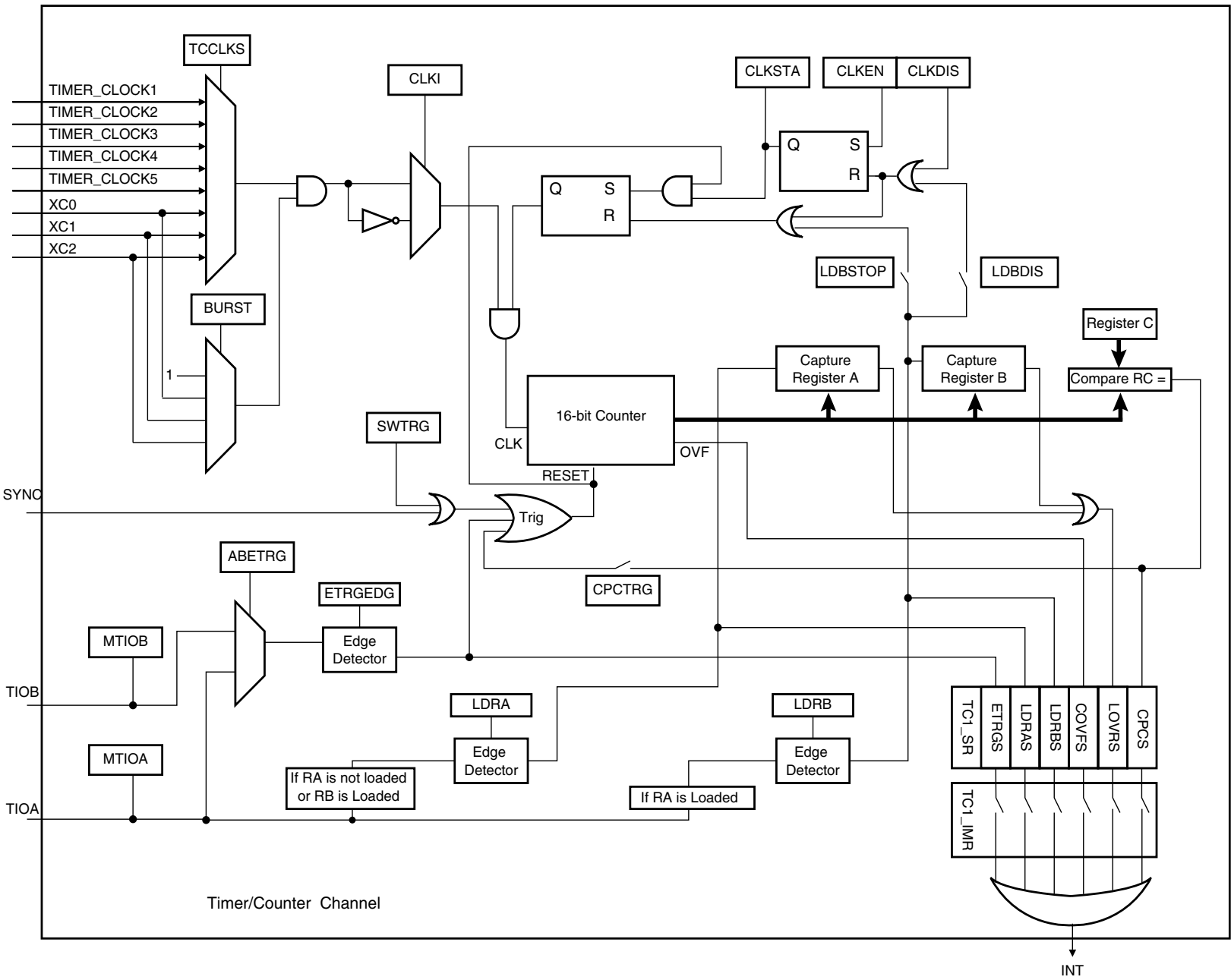
Figure 36-5. Capture Mode
