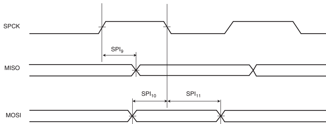
Figure 46-10. SPI Slave Mode with (CPOL = NCPHA = 0) or (CPOL= NCPHA= 1)
