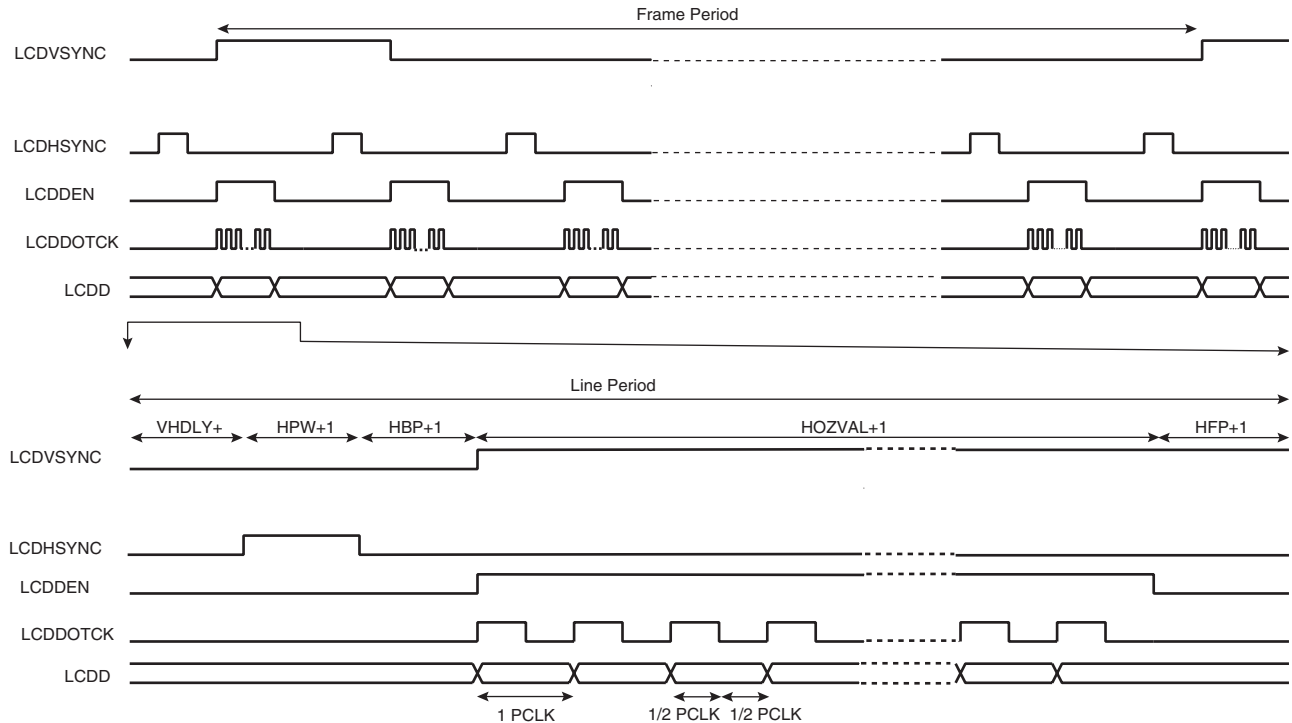
Figure 43-3. STN Panel Timing, CLKMOD 0
