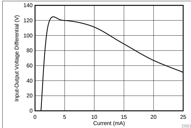
Figure 1. Current Limit
