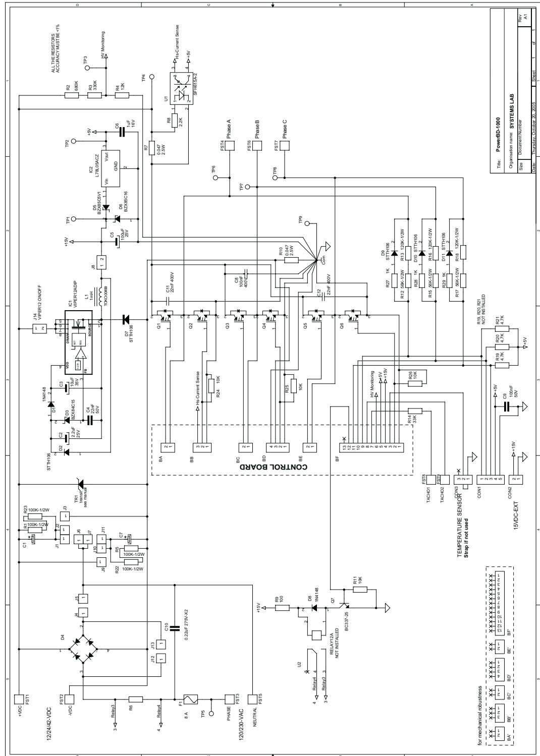
Figure 1. Scheme
