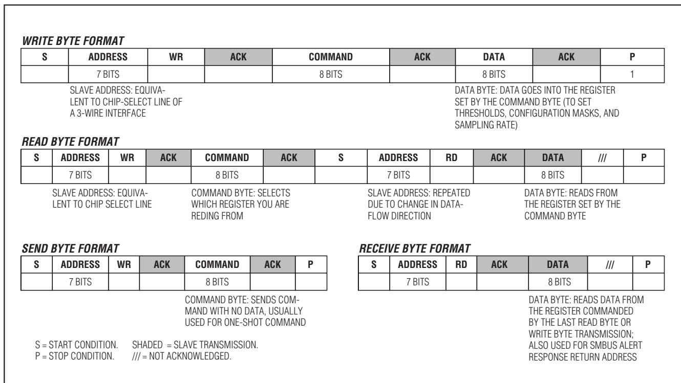
Figure 2. SMBus Protocols
