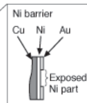
Cross section of contact and post
