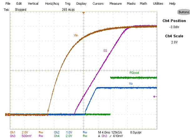
Fig. 18. Start up at 6A Load, Ch_1:V_{in} , Ch_2:V_o , Ch_3:V_{ss} , Ch_4:V_{PGGood}
