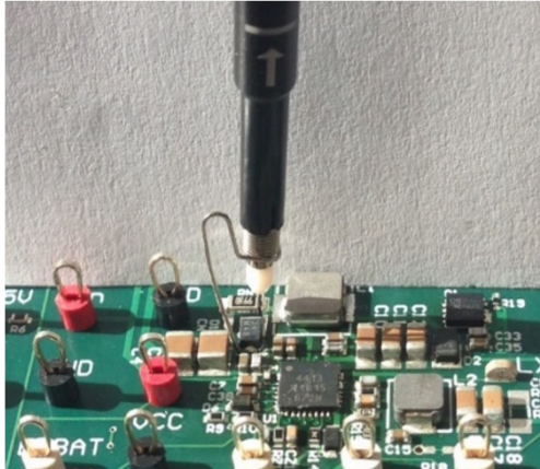
Figure 30: Measuring LX ringing with tip-and-barrel
