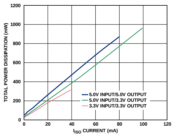
Figure 11. Typical Total Power Dissipation vs. Isolated Output Supply Current in All Supported Power Configurations
