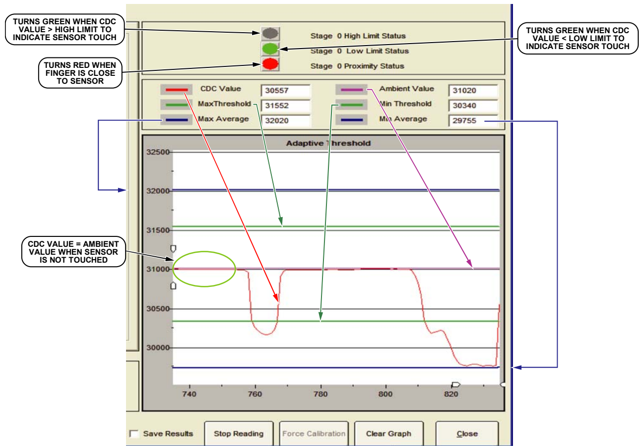
Figure 11. Stage 0 Calibration Engine Dialog Box—Right-Hand Side
