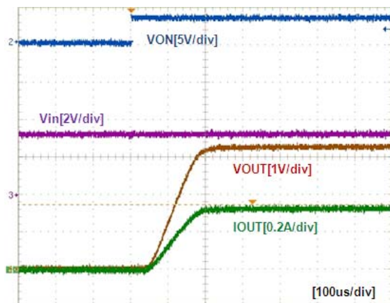
Figure 17. Turn-On Response – FPF1203 / 04 ( V_{IN}=3.3 V, C_{IN}=1 \mu F, C_{OUT}=0.1 \mu F, R_L=10 \Omega )
