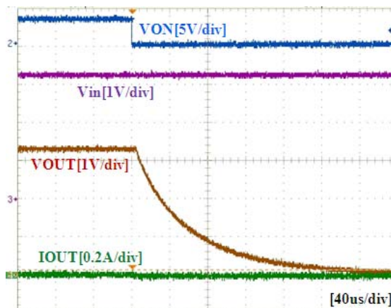
Figure 19. Turn-Off Response – FPF1203 ( V_{IN}=3.3 V, C_{IN}=1 \mu F, C_{OUT}=0.1 \mu F, R_L=500 \Omega )
