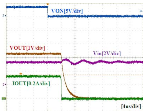
Figure 18. Turn-Off Response – FPF1203 ( V_{IN}=3.3 V, C_{IN}=1 \mu F, C_{OUT}=0.1 \mu F, R_L=10 \Omega )
