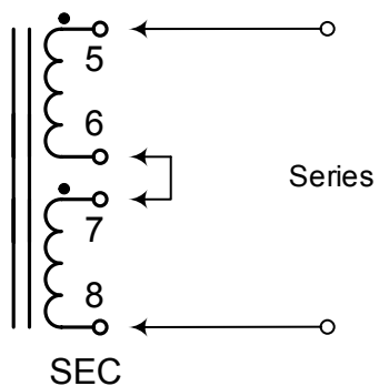
Secondary Wiring (Series Connection)
