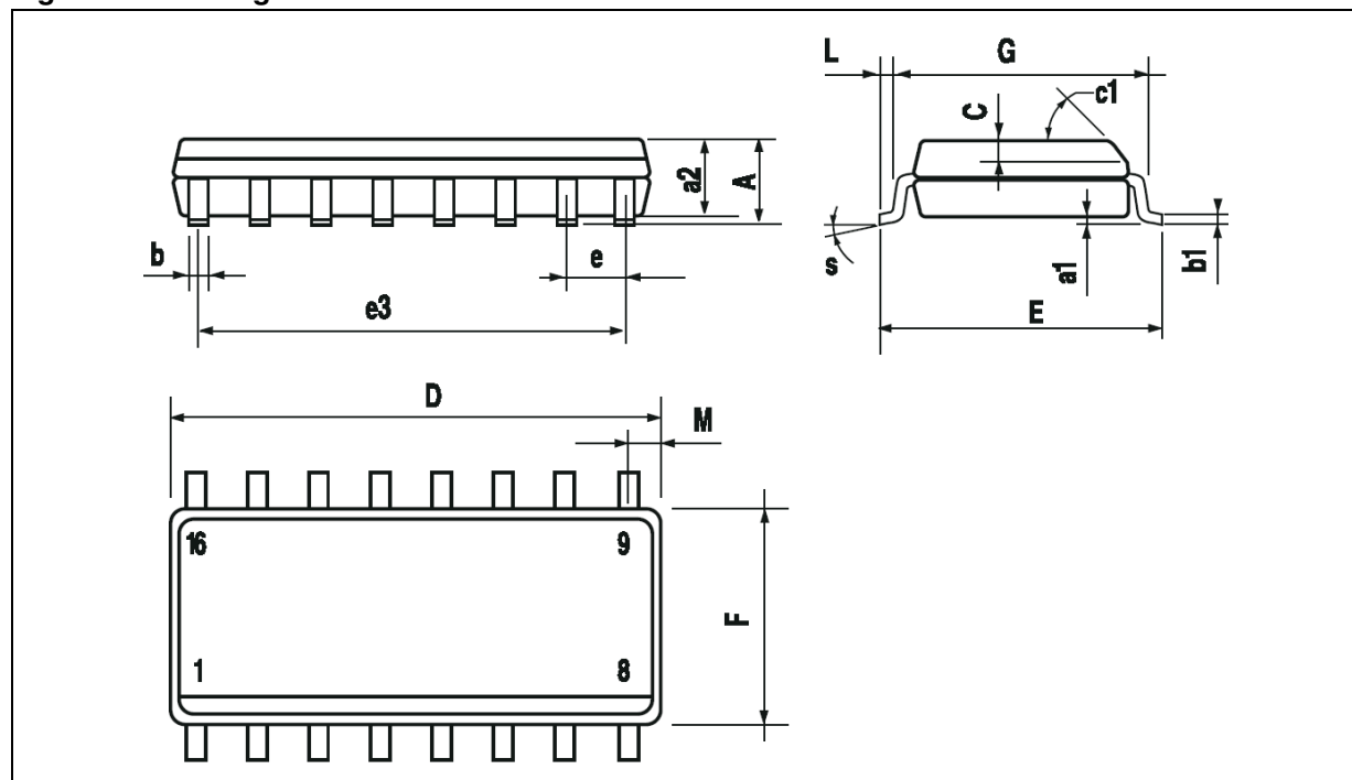
Figure 24. Package dimensions
