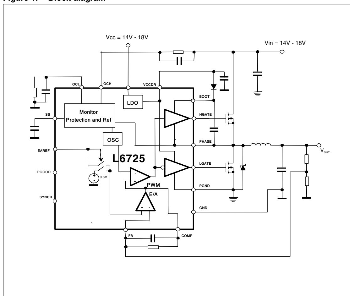
Figure 1. Block diagram
