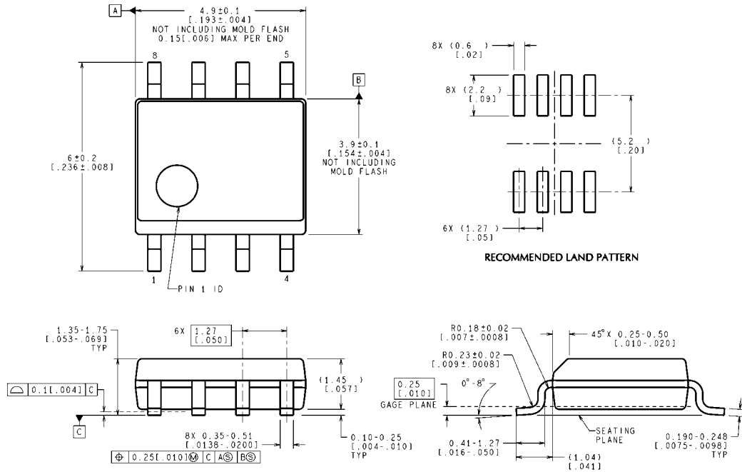
SO-8 Package NS Package Number M08A
