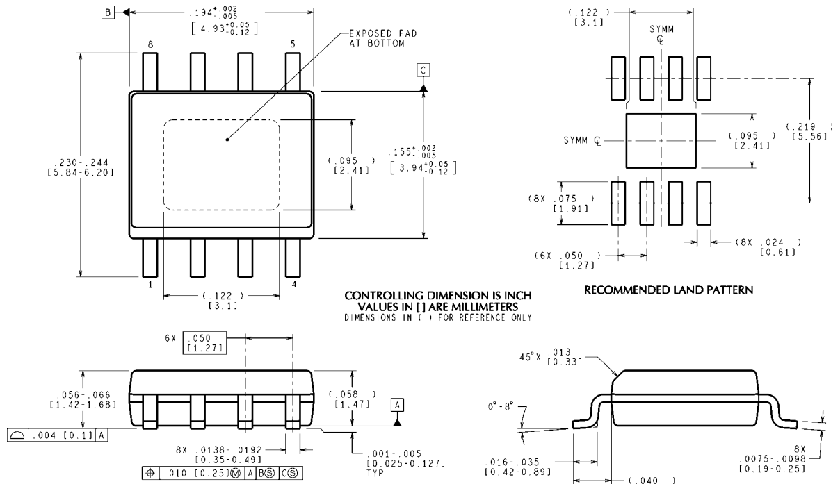
PSOP-8 Package NS Package Number MRA08B
