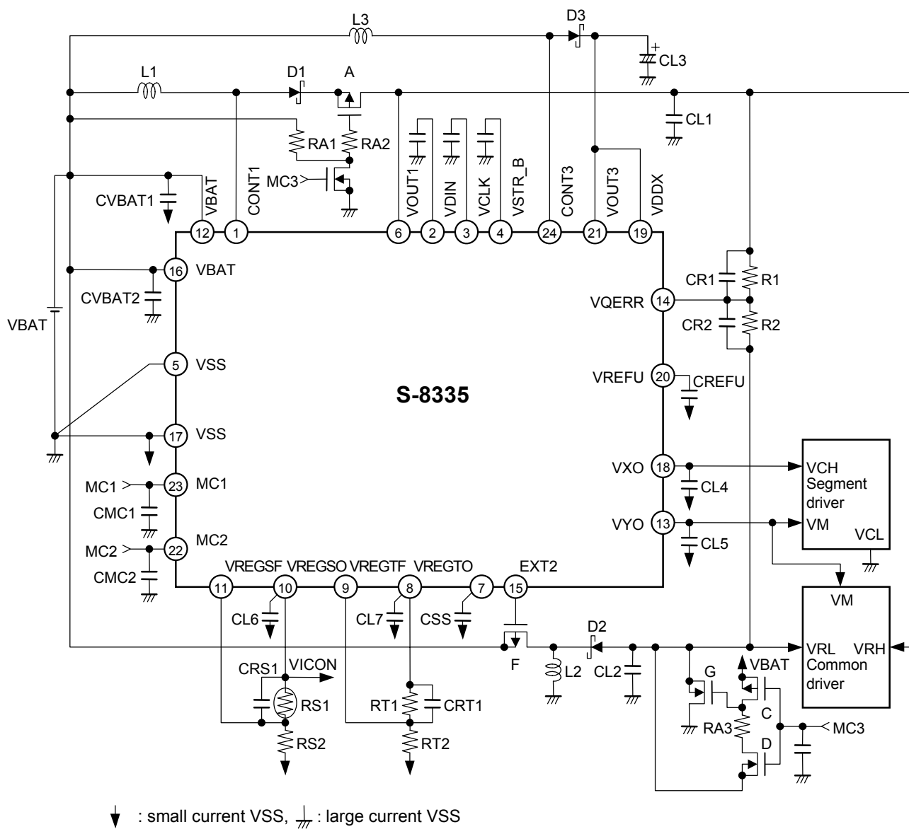
Figure 21 Application Circuit Example
