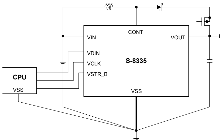
Figure 23 VSS Line
