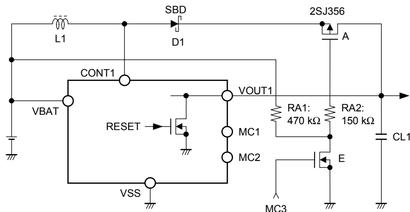
Figure 6 Sample Circuit in Which 2SJ356 is Used
