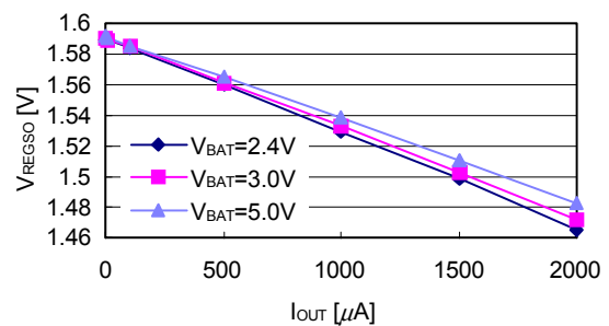
Figure 15 V_{REGSO} Characteristics
