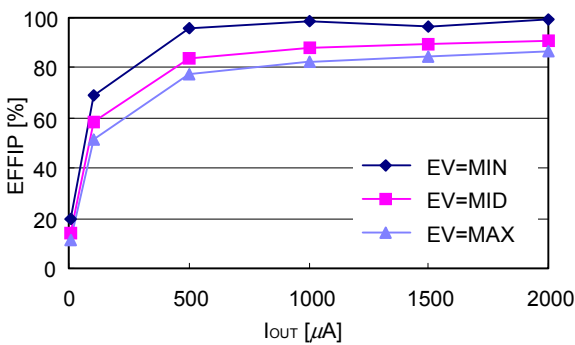
DC/DC P part output efficiency ( V_{BAT} = 5.0 V )
