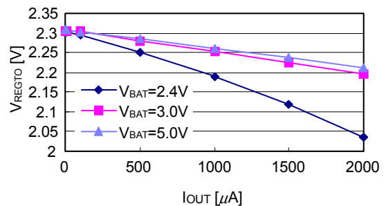
Figure 16 V_{REGTO} Characteristics
