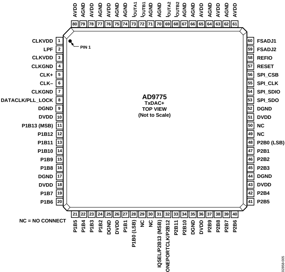
Figure 5. Pin Configuration
