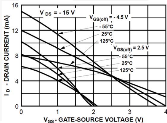
Figure 4. Transfer Characteristics
