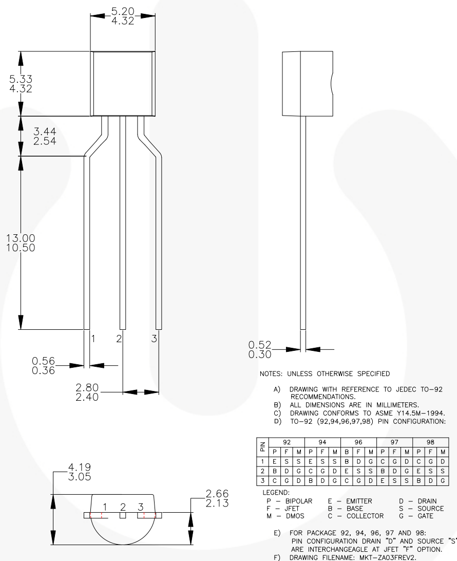
Figure 12. 3-LEAD, TO92, MOLDED, 0.200 IN LINE SPACING LD FORM (J61Z OPTION) (ACTIVE)
