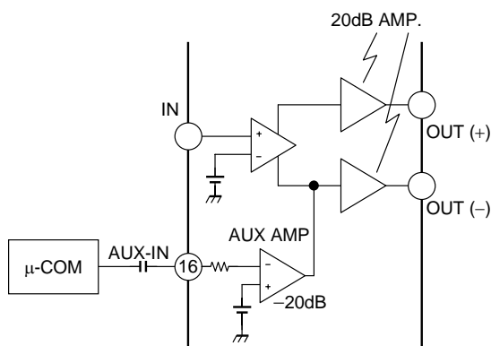
Figure 6 AUX Input
