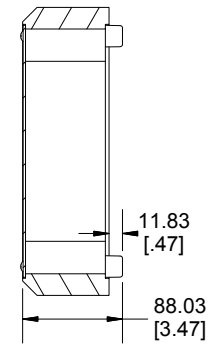
SECTION A-A Without Optional Bottom Panel
