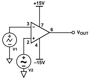
Figure 54. Pulse-Width Modulator
