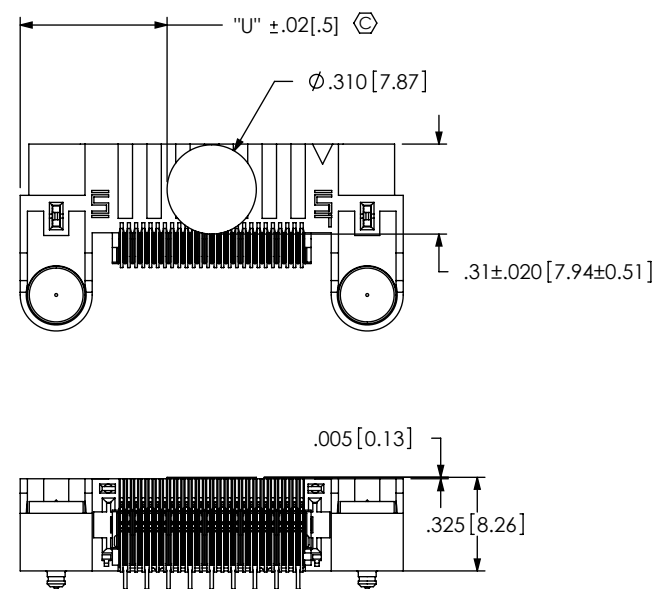
-K: KAPTON PAD QFS-026-01-XX-D-RA-K SHOWN
