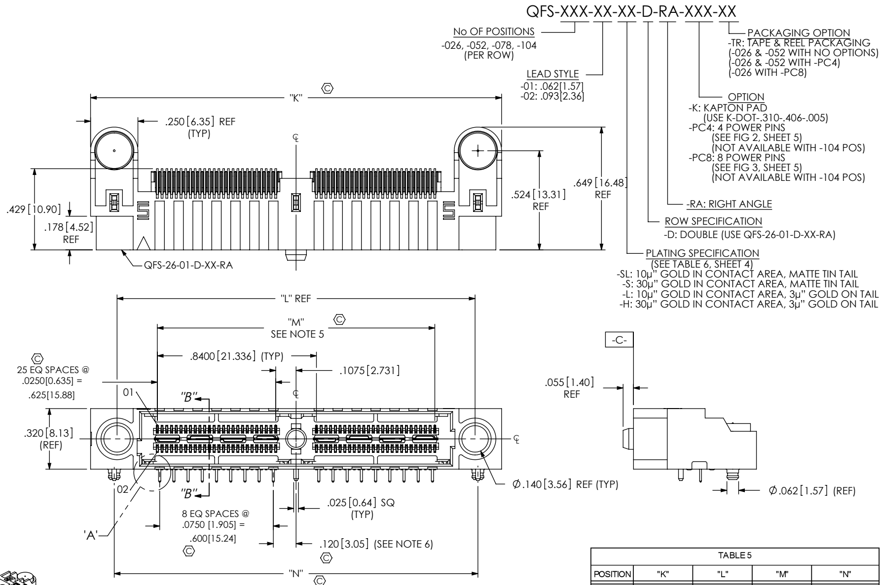
FIG 1 (QFS-052-01-XX-D-RA SHOWN)
