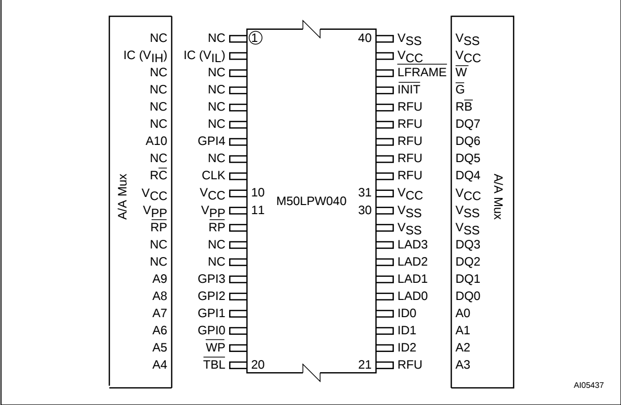
Figure 3. TSOP Connections
