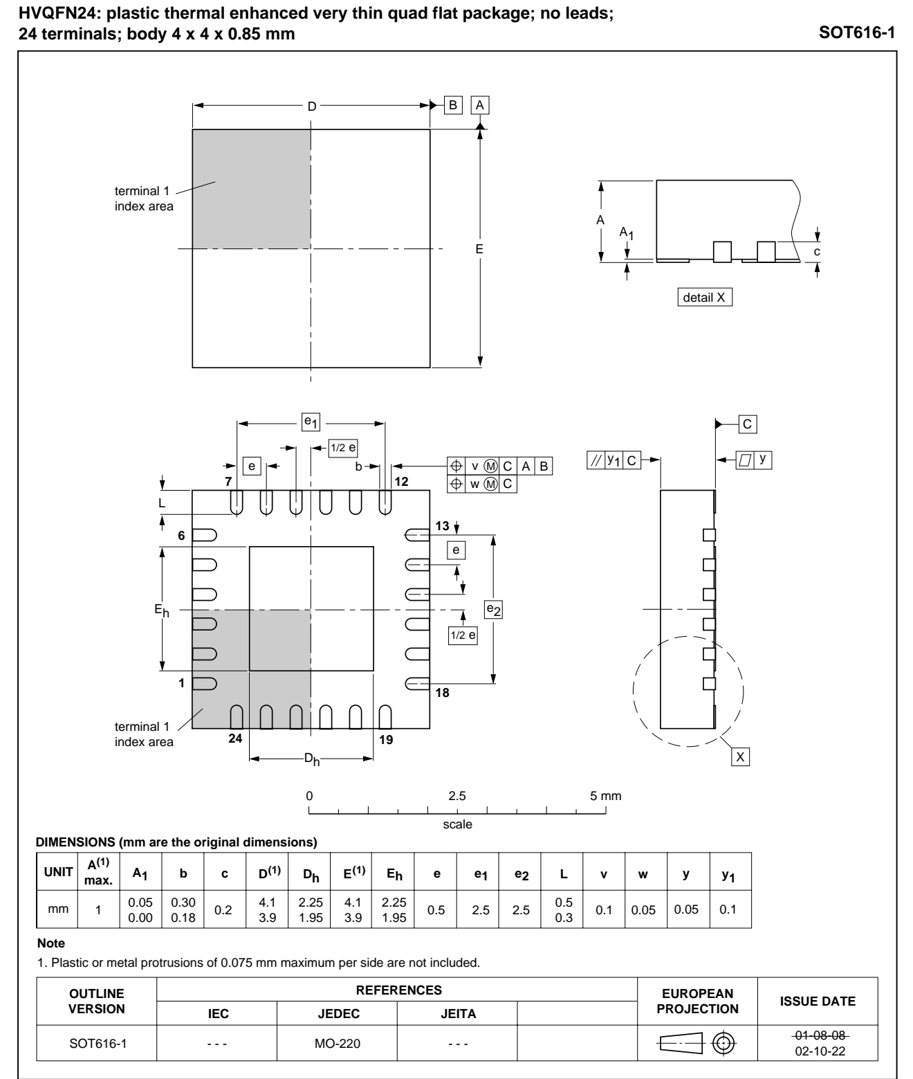
Fig 35. Package outline SOT616-1 (HVQFN24)
