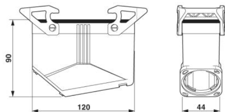
Dimensioned drawing
