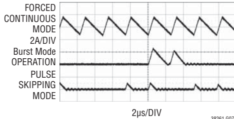
FIGURE 13 CIRCUIT V OUT = 3.3V I LOAD = 100μA
