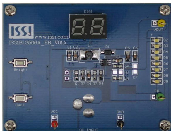
Figure 1: Photo of IS31LT3506A Evalutaion Board
