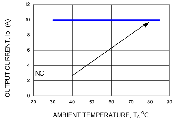
Figure 23. Derating Output Current versus Local Ambient Temperature and Airflow ( V_{in} = 3.3 Vdc, V_o = 2.5 Vdc).
