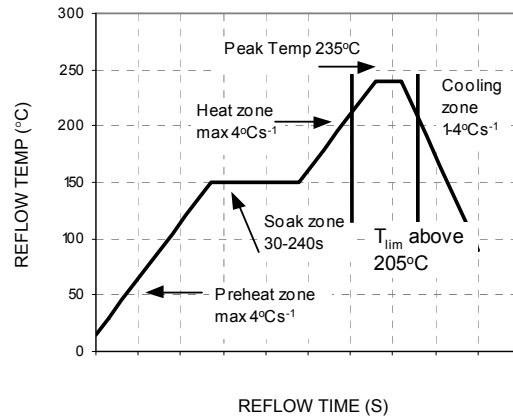
Figure 36. Reflow Profile for Tin/Lead (Sn/Pb) process.
