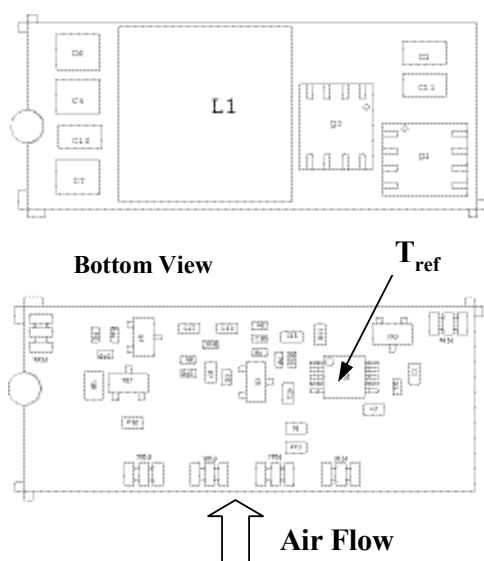
Figure 34. T ref Temperature measurement location.
