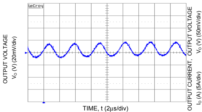
Figure 9. Typical Output Ripple and Noise ( V_{IN} = 5.0V dc, V_O = 3.3 Vdc, I_O = 10A ).
