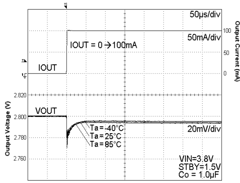
Fig. 52 Load Response
