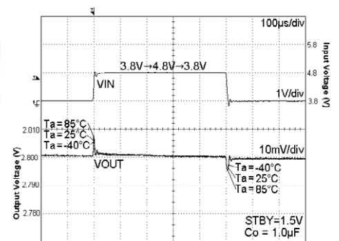
Fig. 65 VIN Response Iout = 10mA
