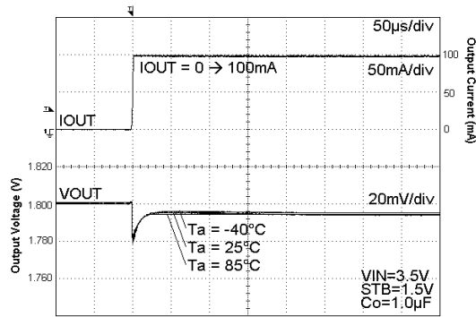
Fig. 81 Load Response
