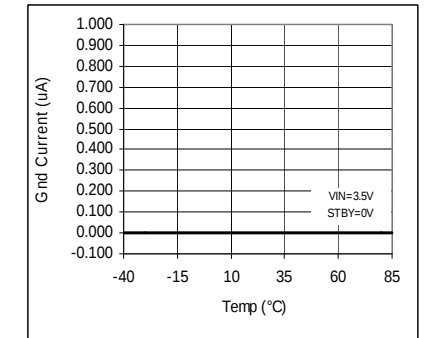
Fig. 77 IGND vs. Temp (STBY)
