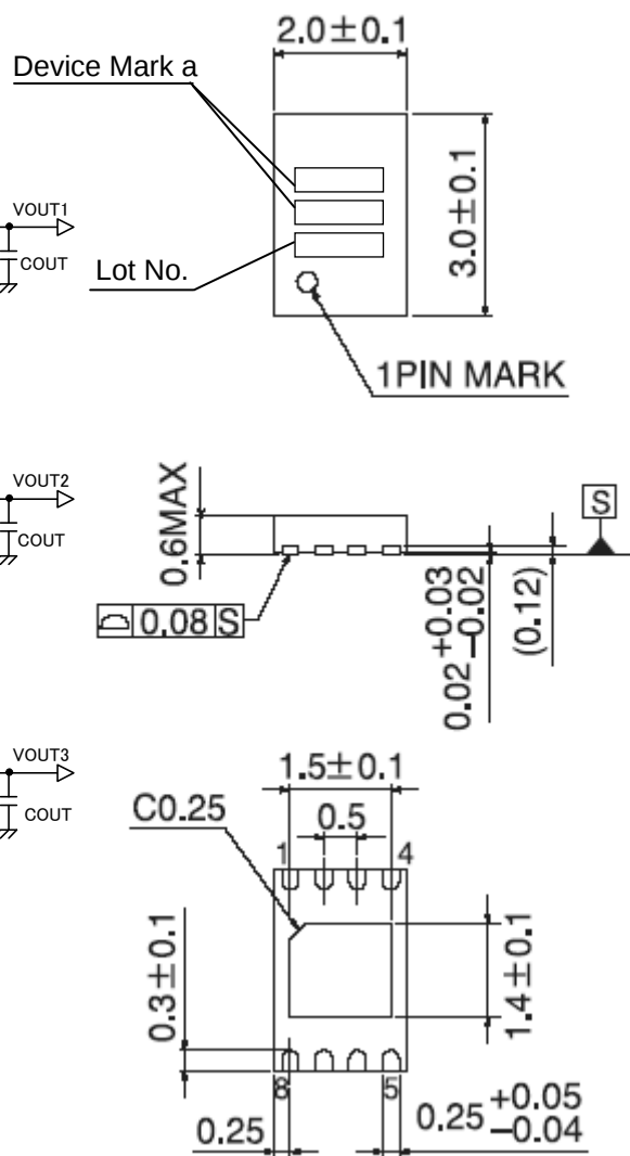
Fig.2 Package dimensions
