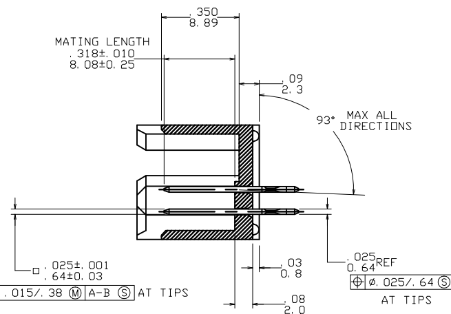
SECTION Y-Y
