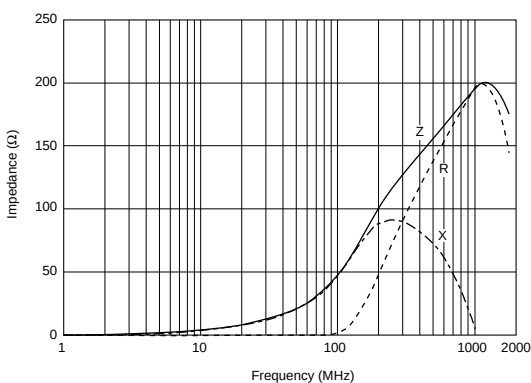
BLM18BB470SH1
