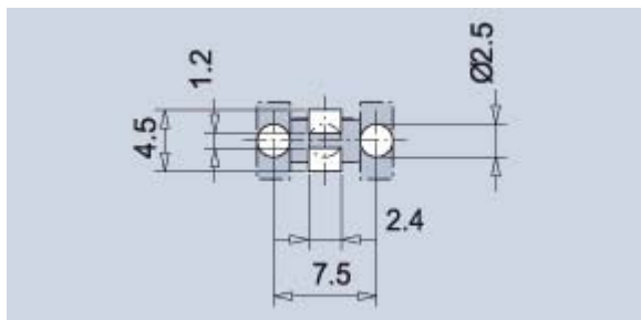
Layoutvorschlag · Layout Suggestion
