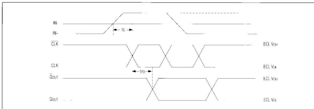
Figure 2. Timing Diagram
