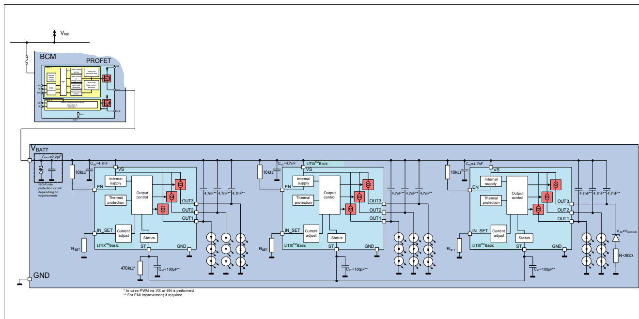
Figure 20 System Diagram TLD1313EL in combination with mutiple devices and two channel usage for device at the right side
