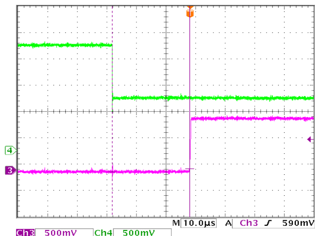
FIGURE 6. ISL88003 t_{PRD} ~26μs
