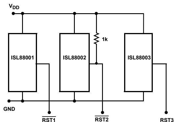
FIGURE 13. ISL88001/2/3EVAL1Z SCHEMATIC
