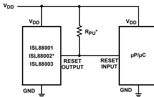
FIGURE 1. TYPICAL APPLICATION DIAGRAM
