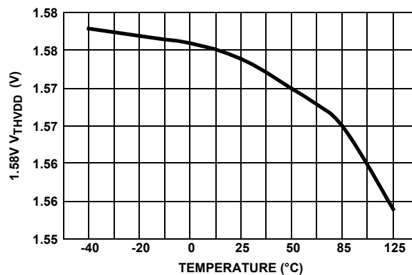
FIGURE 10. ISL8800x 1.58V V_{THVDD} vs TEMPERATURE
