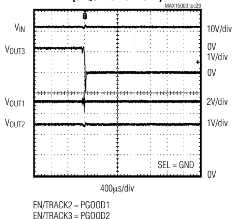
IN-PHASE OPERATION
