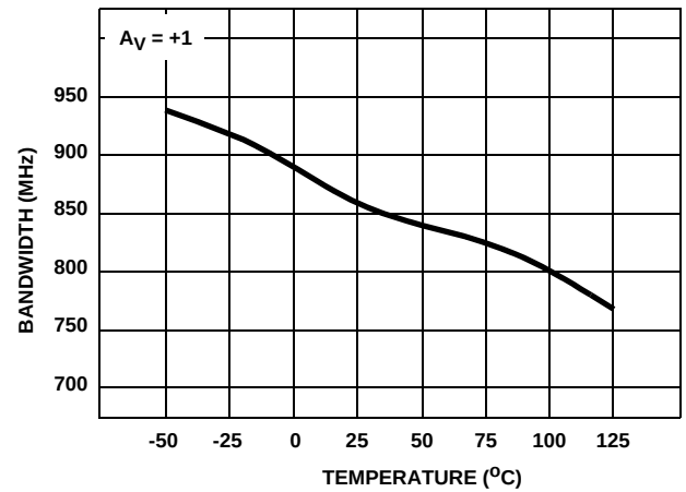
FIGURE 10. -3dB BANDWIDTH vs TEMPERATURE
