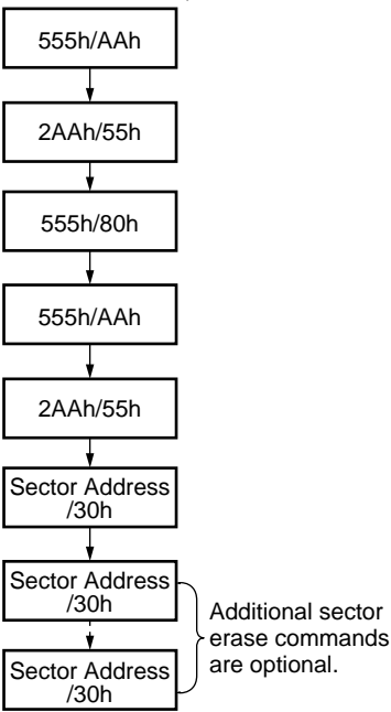
Individual Sector/Multiple Sector Erase Command Sequence (Address/Command):
