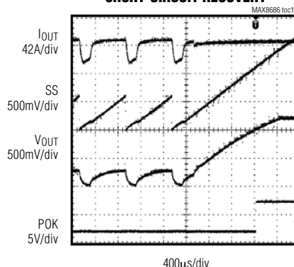
SHORT-CIRCUIT RECOVERY
