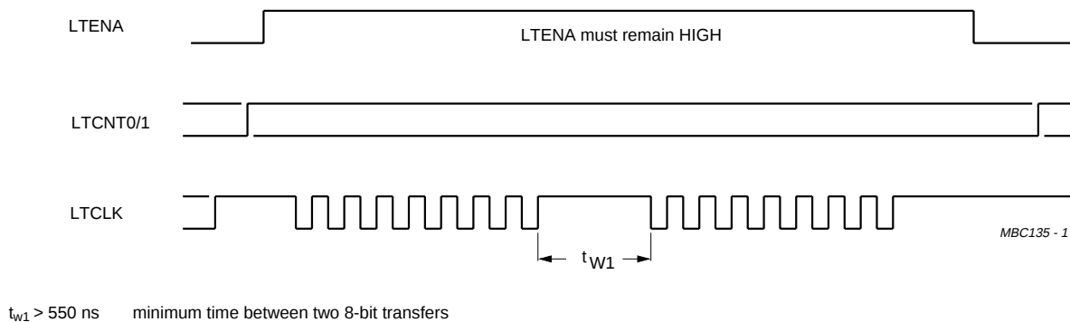
Fig.16 16-bit transfers.
