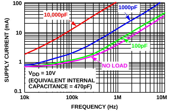
FIGURE 8. AVERAGE SUPPLY CURRENT vs CAPACITIVE LOAD
