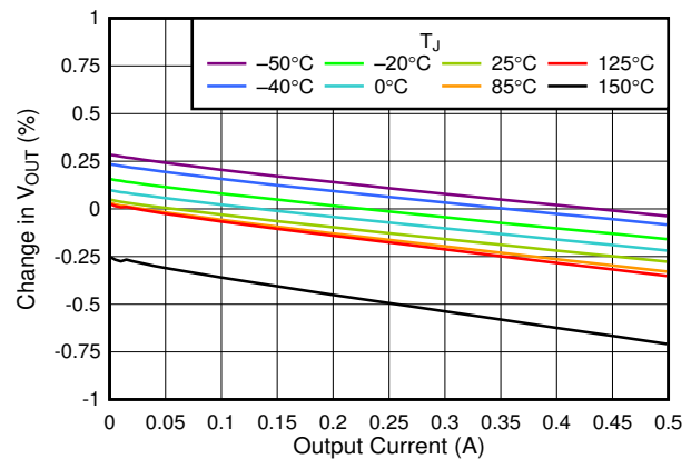
Figure 6-18. 5.5-V Load Regulation vs I_{OUT}
