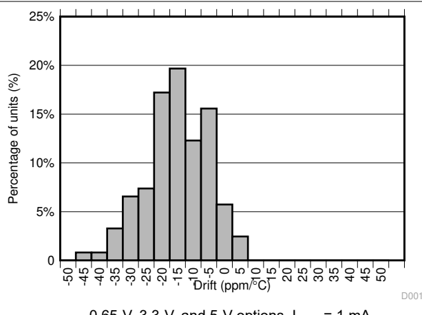
Figure 6-4. Temperature Drift Histogram ( -40^\circ\text{C} to +25^\circ\text{C} )
