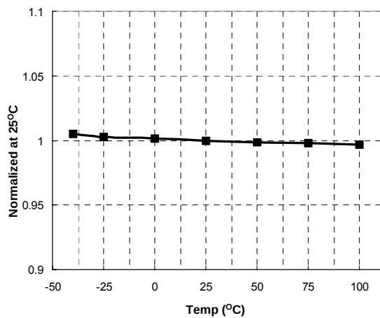
Figure 9. Low-Side V_{CC} ( LV_{CC} ) Stop vs. Temperature
