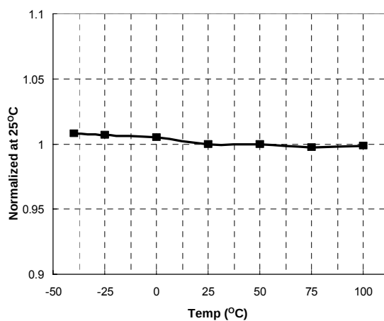
Figure 7. High-Side V_{CC} ( HV_{CC} ) Stop vs. Temperature
