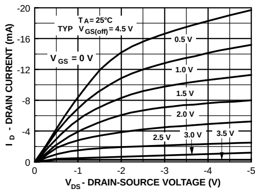
Common Drain-Source
