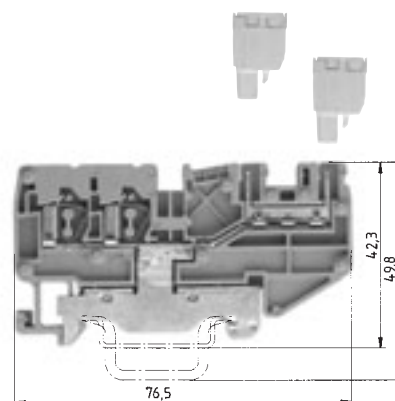
finely stranded single core V A 0.13 – 2.5 mm 2 0.13 – 4 mm 2 250 V/4 kV/3 16 No. 22 – 12 AWG 300 No. 24 – 12 AWG 300 5 mm 11 mm
