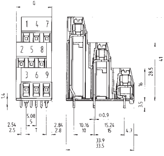
with insulating plate, with locating cams
