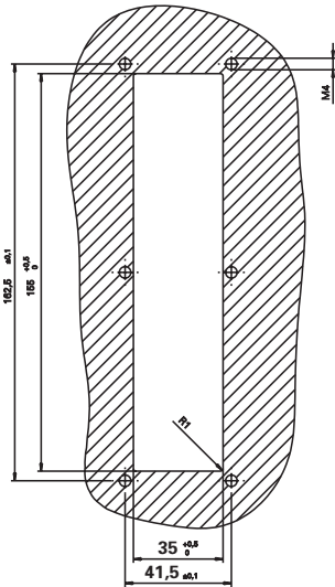
Overall dimensions, steel cutout and drill hole configuration are identical for all TM6 variants
