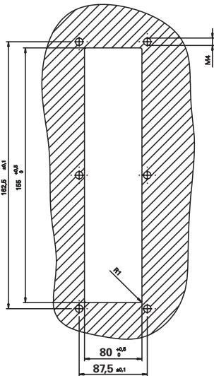
Overall dimensions, steel cutout and drill hole configuration are identical for all 6 variants
