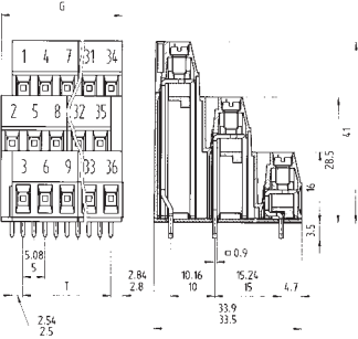
with insulating plate, without locating cams
