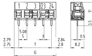
with insulating plate
