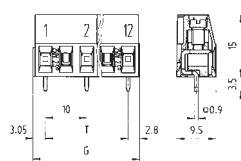
pitch 10.00 mm, without insulating plate
