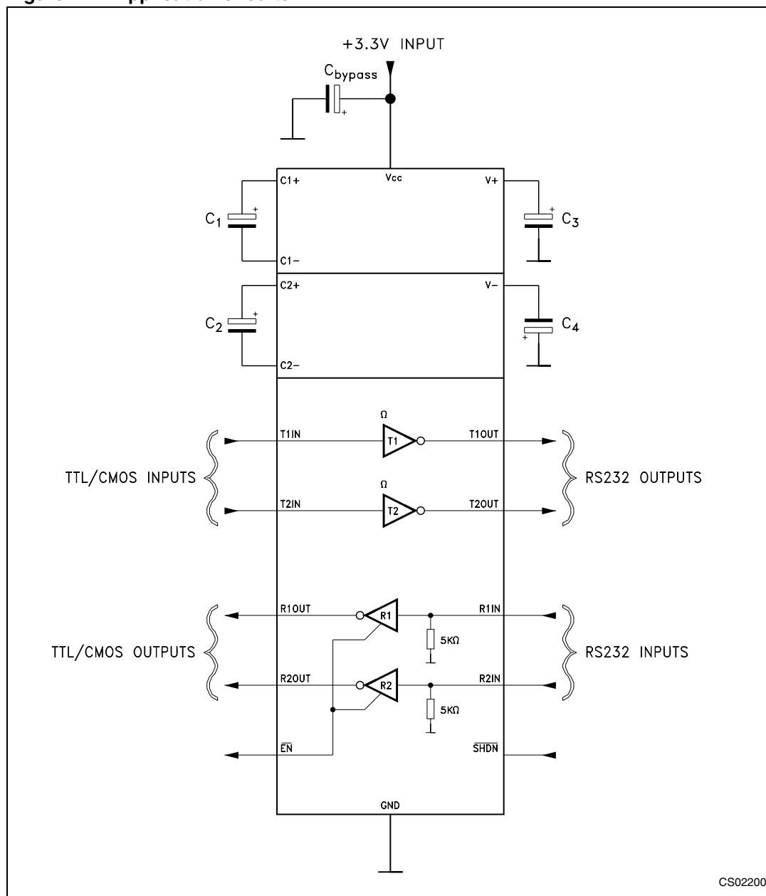
Figure 2. Application circuits
