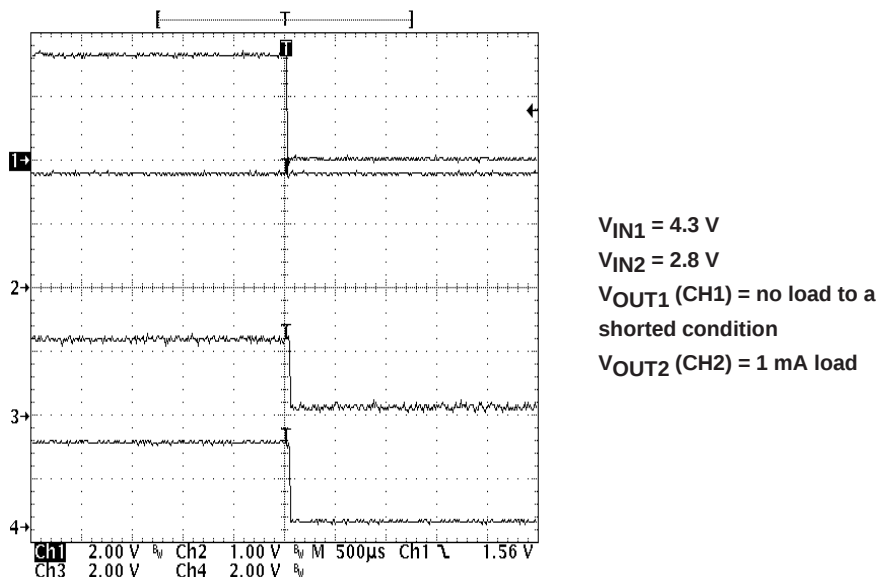
Figure 4–7. Timing When SEQUENCE Is High, With a Fault on V_{OUT1}
