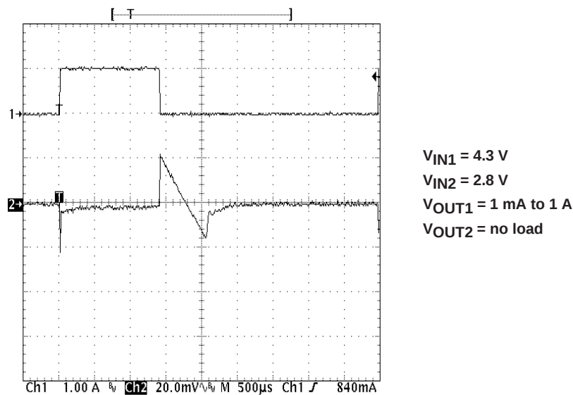
Figure 4–1. V_{OUT1} Load Transient
