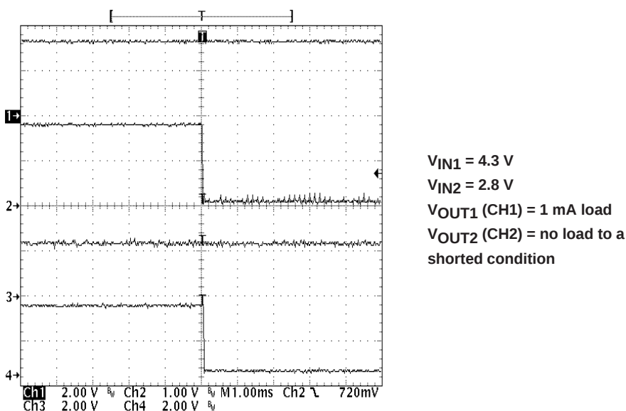
Figure 4–8. Timing When SEQUENCE Is Low, With a Fault on V_{OUT2}
