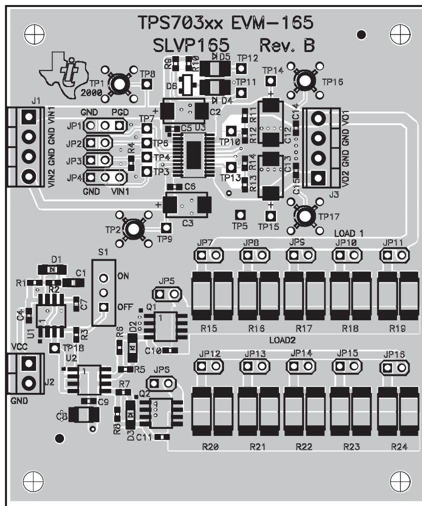
Top Assembly
