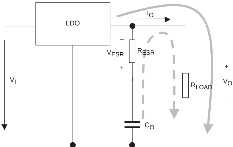
Figure 3–2. LDO Output Stage With Parasitic Resistances ESR
