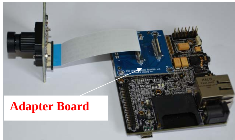
Camera Modules with Leopardboard 36x through Adapter board
