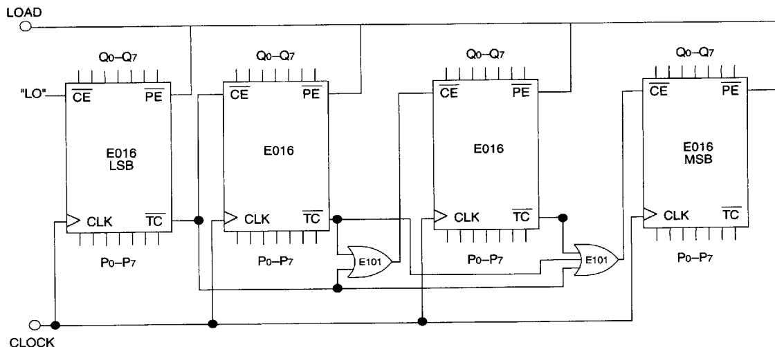
Figure 1. 32-Bit Cascaded E016 Counter
