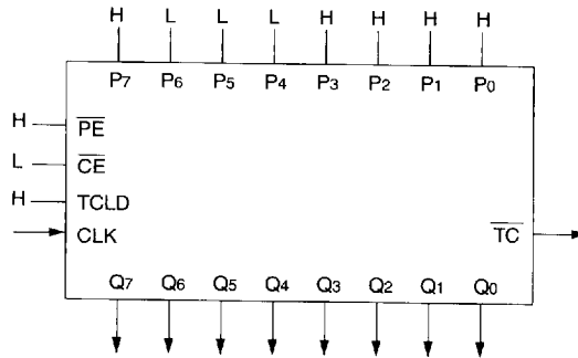
Figure 2. Mod 2 to 256 Programmable Divider
