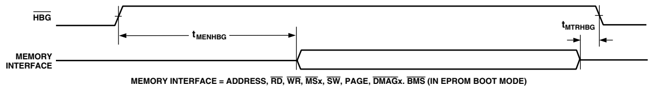
Figure 19b. Three-State Timing (Host Transition Cycle)
