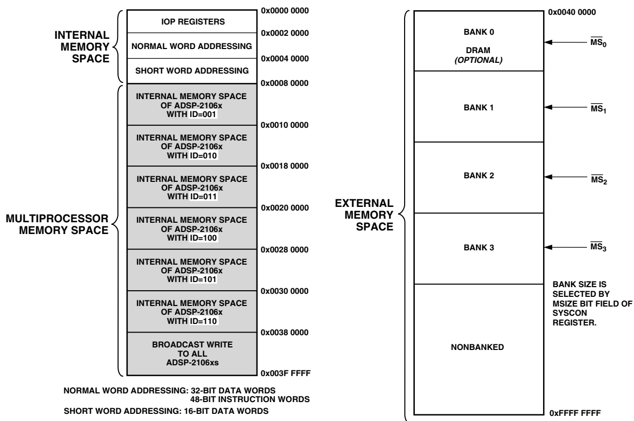
Figure 4. ADSP-21061/ADSP-21061L Memory Map
