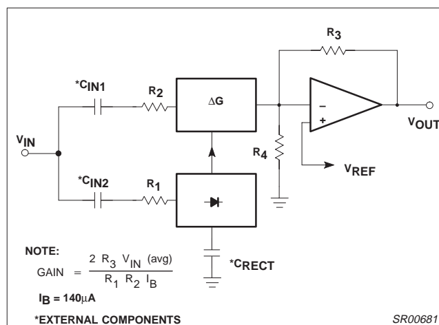
Figure 7. Basic Expander
