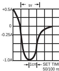
FIG. 5 - TEST CIRCUIT DIAGRAM AND REVERSE RECOVERY TIME CHARACTERISTIC
